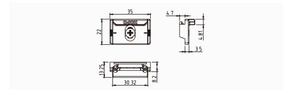
C groove adjustable locking plate AALP10
