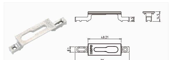
Locking plate SLP47.00
