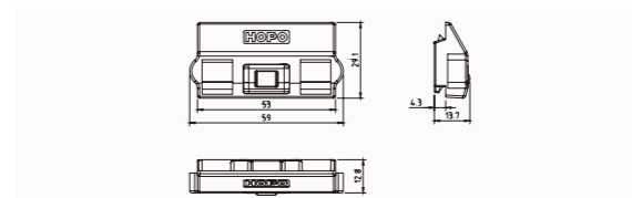
K groove sash support device ASP30.00
