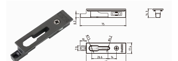
Locking plate SLP47.03
