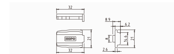
Anti-dropping block AAS10
