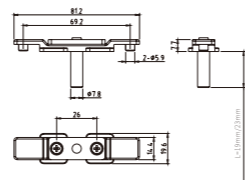
Heavy-duty T-type connector TTC31
