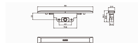
Gear case AGC36.23
