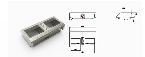
K groove adjustable locking plate ASLP20.05
