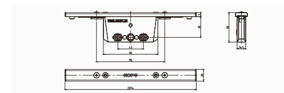
FM30 Gear case AGC31.35
