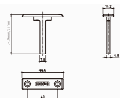
Heavy-duty T-type connector TTC29
