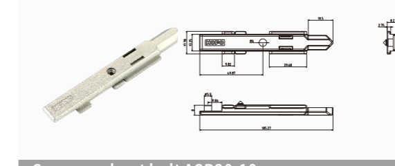
C groove shoot bolt ASB20.10
