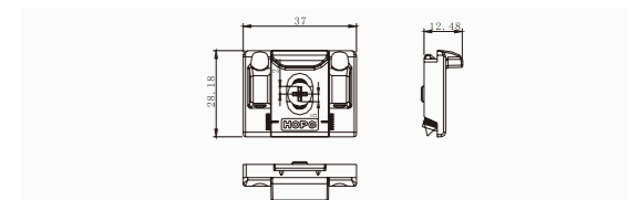
K groove adjustable locking plate AALP20
