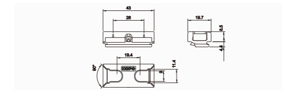
C groove locking plate ALP33
