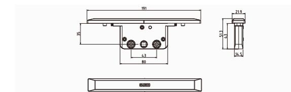
Gear case AGC36.35
