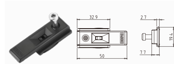
Sliding rod LPE45.07
