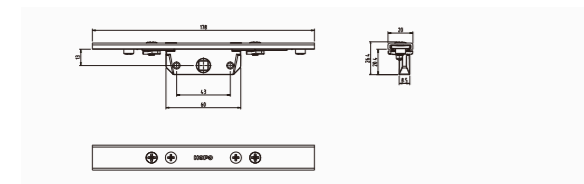
Gear case AGC34.13.011H5
