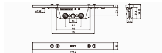
FM18 Gear case AGC31.23
