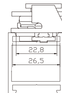
K groove friction hinge FH07
