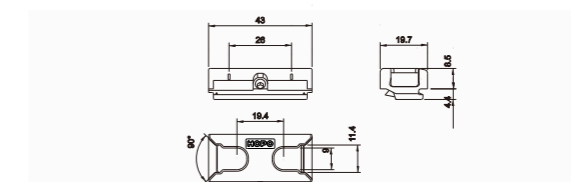
C groove locking plate ALP33
