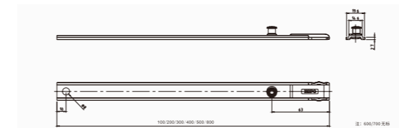
Transmission rod DR21
