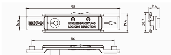
Locking rod ALR10
