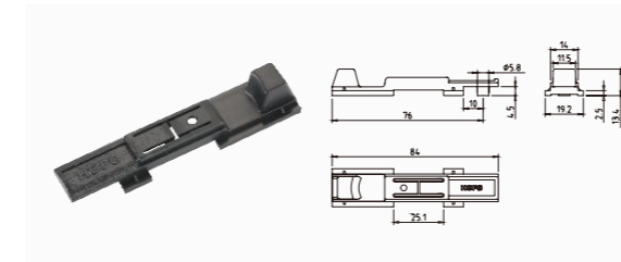
C groove shoot bolt driver ASBH20.00
