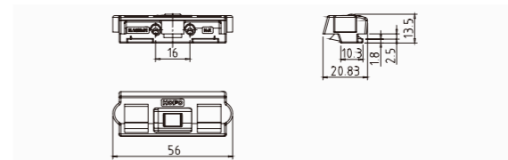
Sash support device ASP20.00
