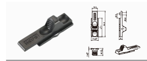
C groove shoot bolt driver ASBH20.10
