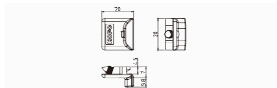
C groove locking plate ALP10 Stock
