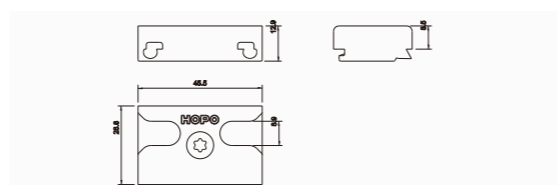
K groove stainless steel locking plate ALP17
