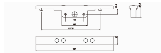
Gear case AGC32.13
