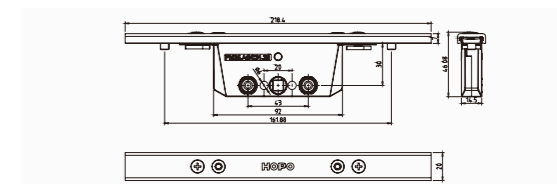
FM25 Gear case AGC31.30
