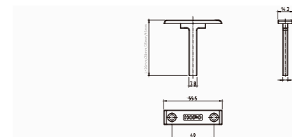
Heavy-duty T-type connector TTC29
