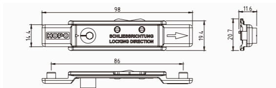
Locking rod ALR10 Stock
