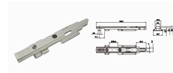
C groove shoot bolt ASB20 Stock
