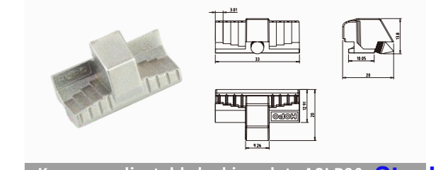
K groove adjustable locking plate ASLP20 Stock
