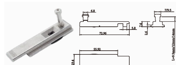
Sliding rod LPE46.07
