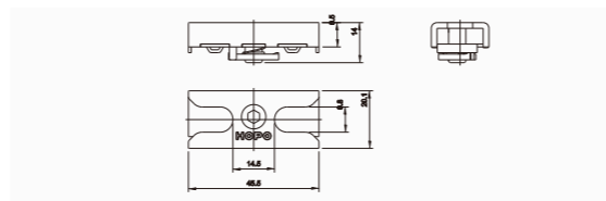
C groove stainless steel locking plate ALP23
