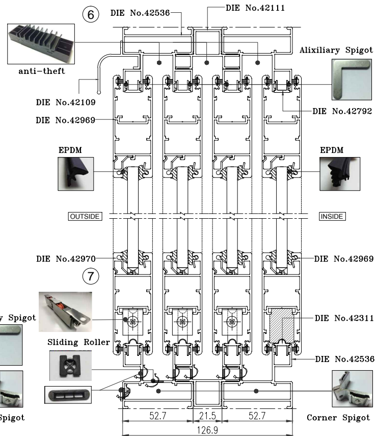
SECTION-B VERTICAL SECTION DETAIL
