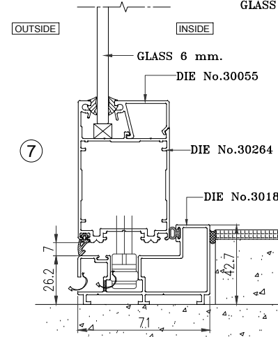
SECTION-B VERTICAL SECTION DETAIL
