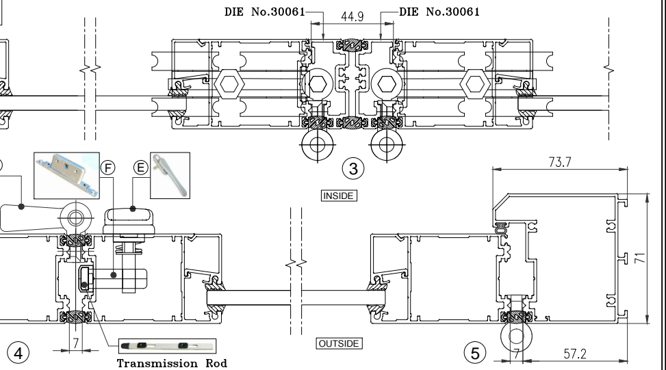
SECTION-B VERTICAL SECTION DETAIL
