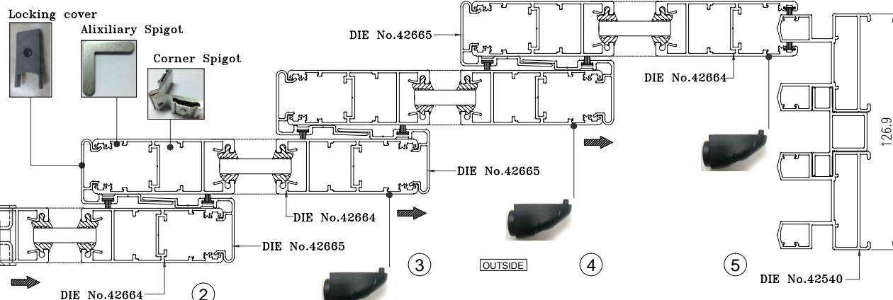
SECTION-A HORIZONTAL SECTION DETAIL
