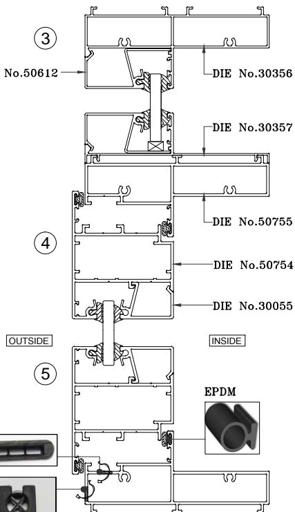
CASEMENT WINDOW (Euro)
