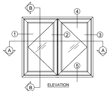
DOUBLE CASEMENT WINDOW (Euro)
