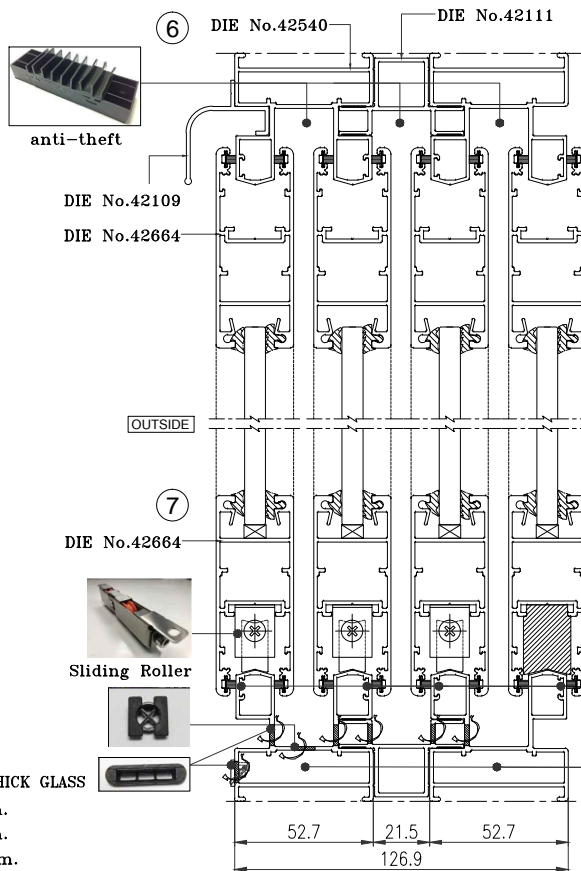
SECTION-B VERTICAL SECTION DETAIL
